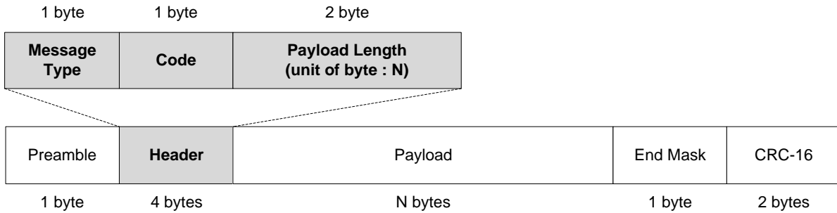
Figure 8 RCP packet format
