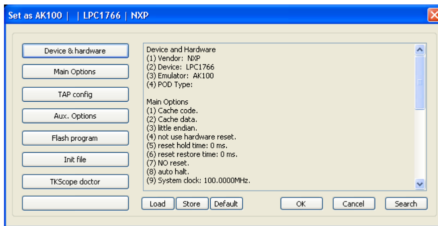
Figure 4.6 AK100 emulator settings interface
