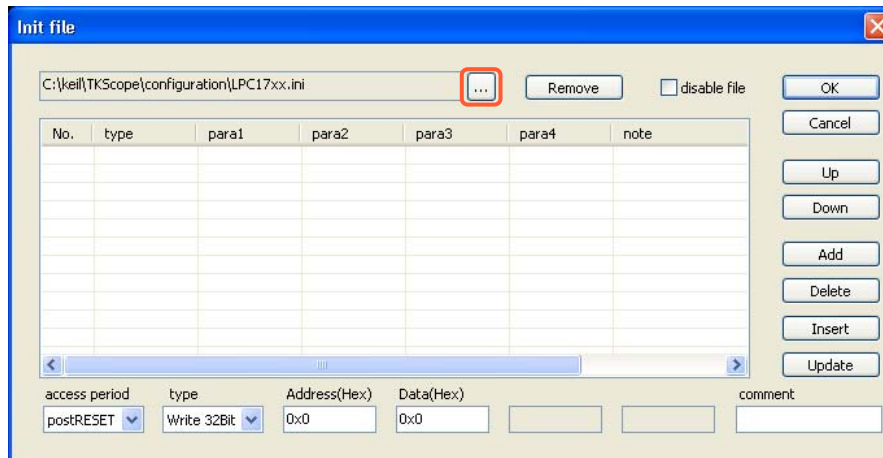
Figure 3.11 Init File Interface
