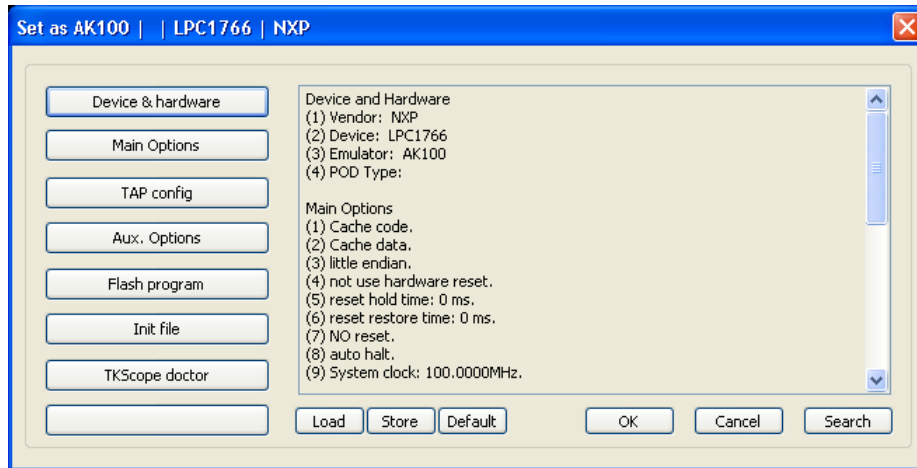
Figure 5.9 AK100 emulator settings interface
