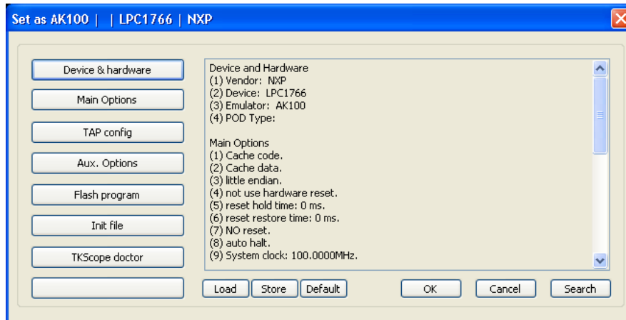
Figure 6.5 AK100 emulator settings interface
