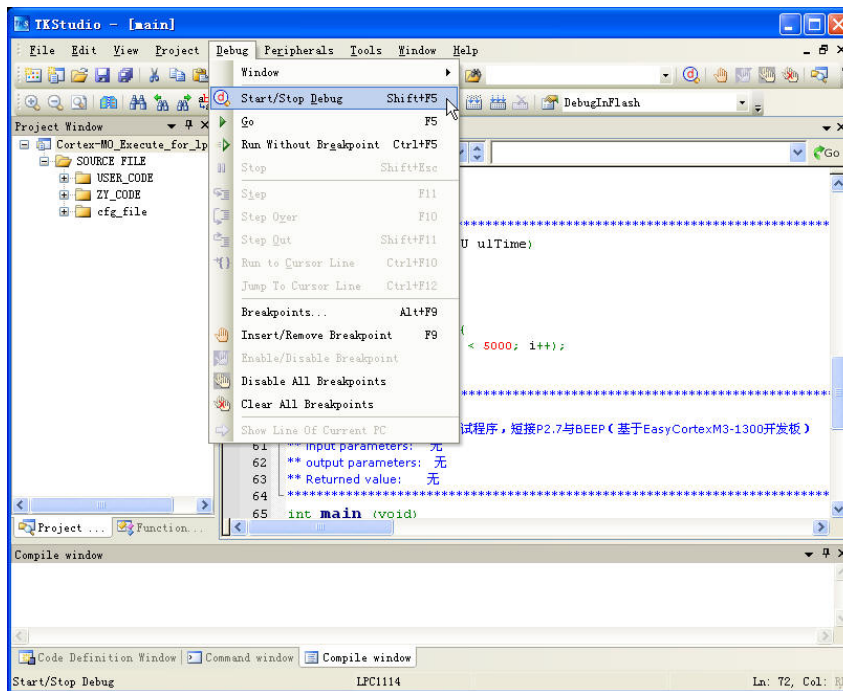
Figure 6.6 Start Debugging
