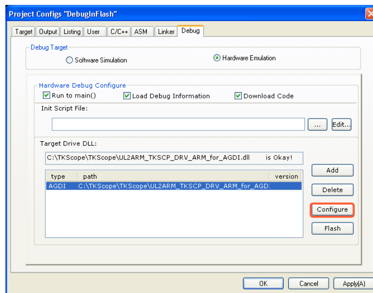
Figure 6.4 Driver file installed
